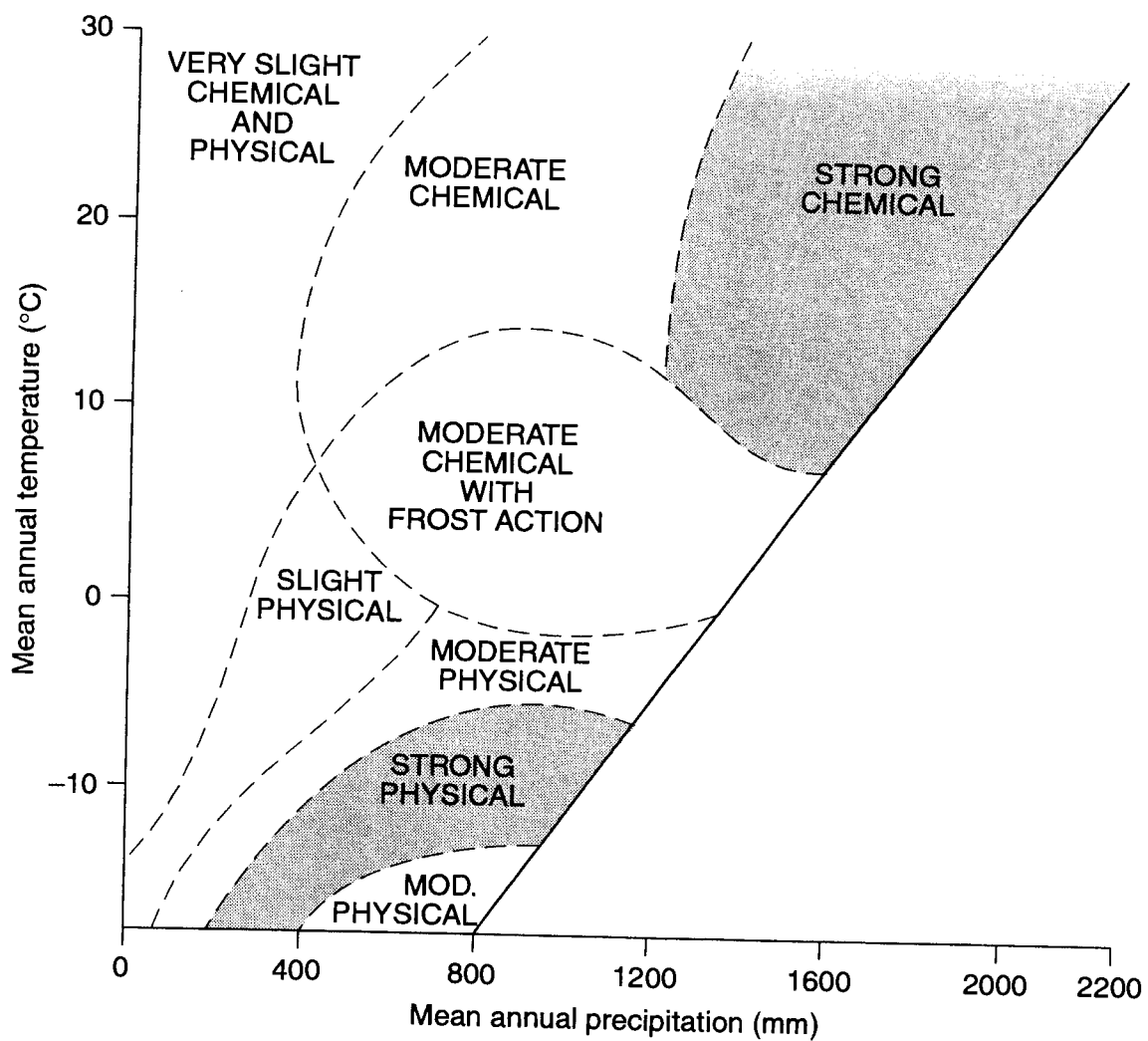
Fig 2. Peltier Diagram
